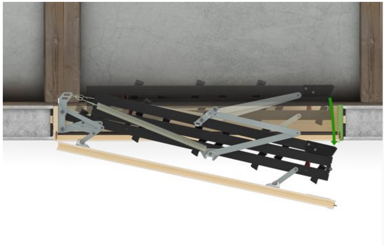
Figure 2. Swing space of the loft ladder equipped with the LXS-M stile ends
